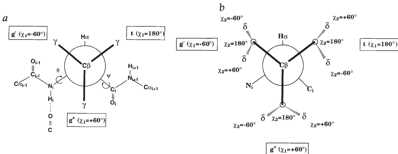
Fig. 2 Newman projections of a, the backbone conformation dependent interactions of protein sidechains with the backbone and b, the backbone conformation independent interactions of protein sidechains with the backbone.
