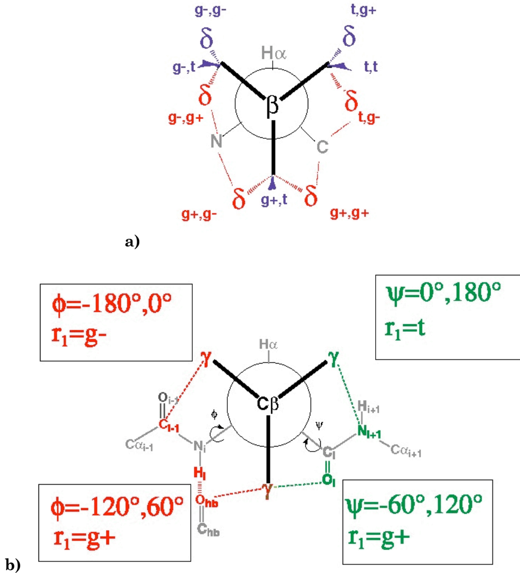
Figure 2. Newman projections of (a) the backbone conformation dependent interactions of protein sidechains with the backbone and (b) the backbone conformation independent interactions of protein sidechains with the backbone.
