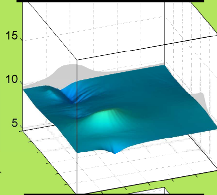
20 ARG: \sigma_{\chi_1}(\phi, \psi | r = \langle g^-, g^-, t, t \rangle) , 2.76%
